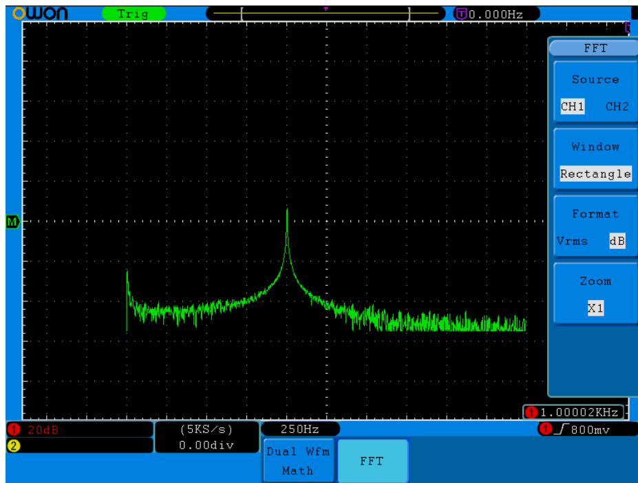
Fig.5-8. Rectangle window
