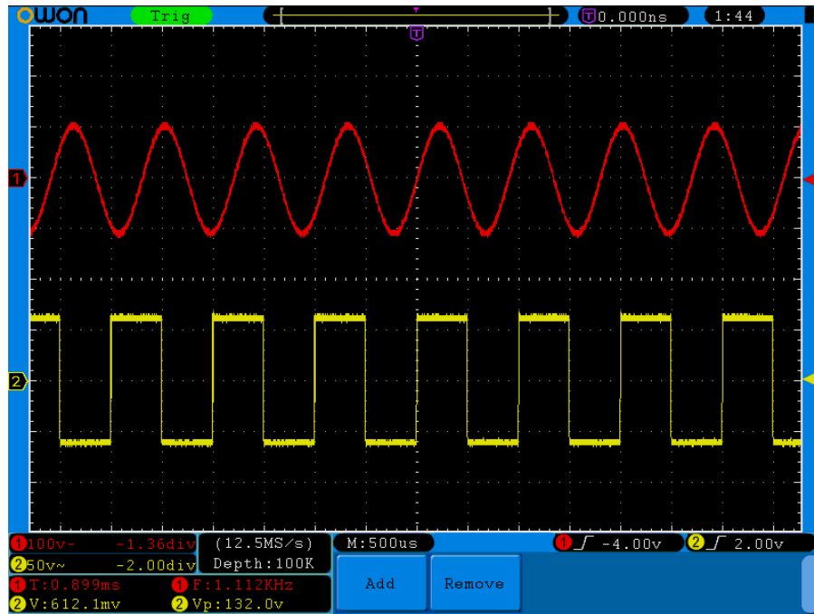
Fig.5-48 automatic measurement
