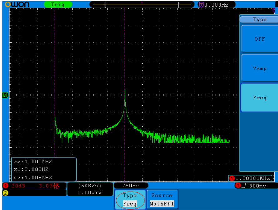
Fig.5-56 wave of Freq cursor measurement
