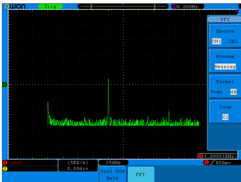
Fig.5-10 Hanning window
