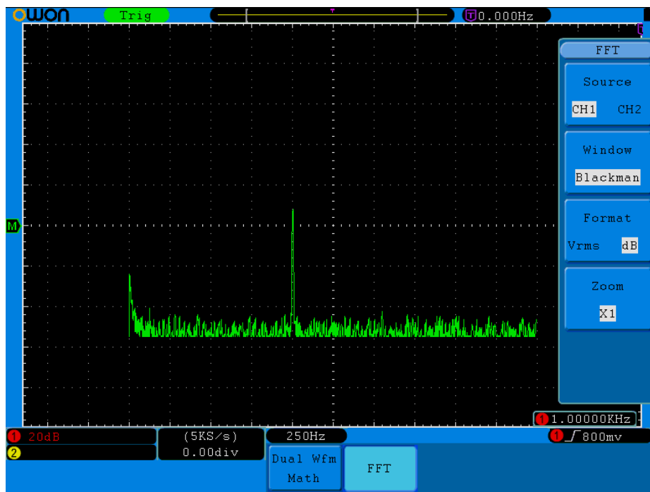
Fig.5-11. Blackman window
