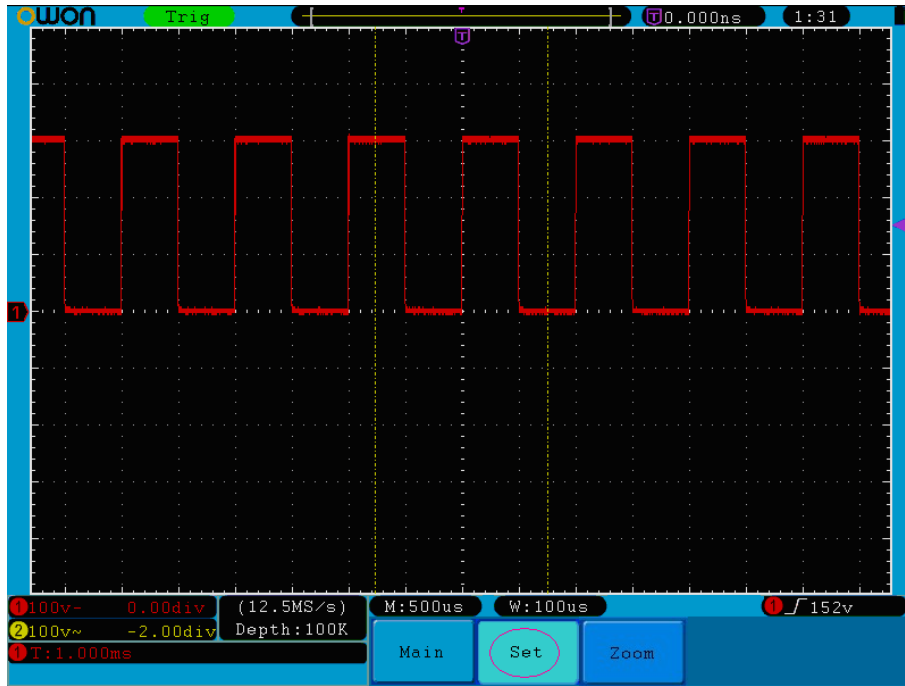
Fig. 5-15 Window Setting
