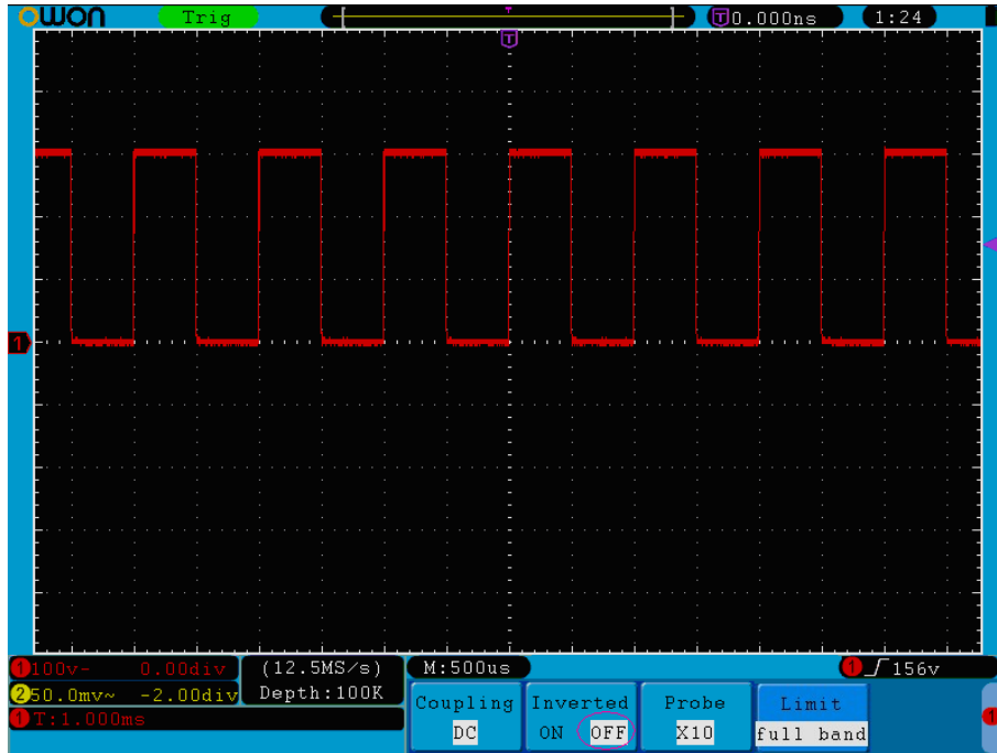
Fig. 5-4 Original Waveform
