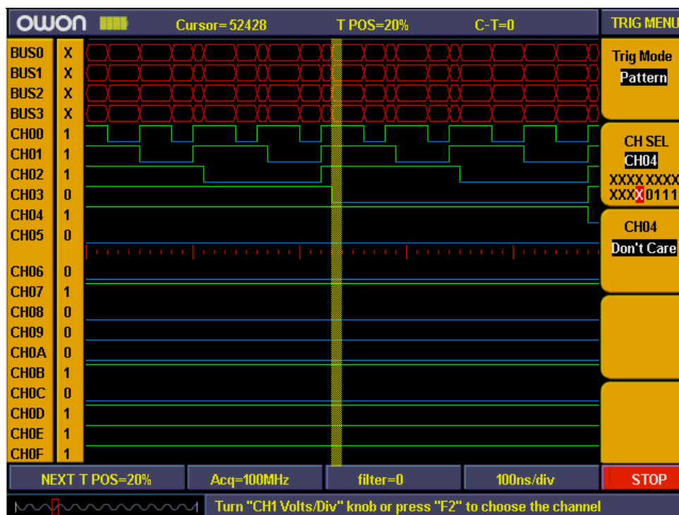
Fig 67: Pattern trigger
