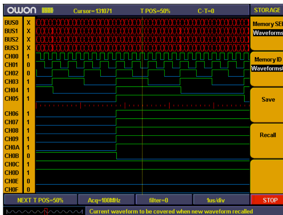
Fig 82: Waveform saving
