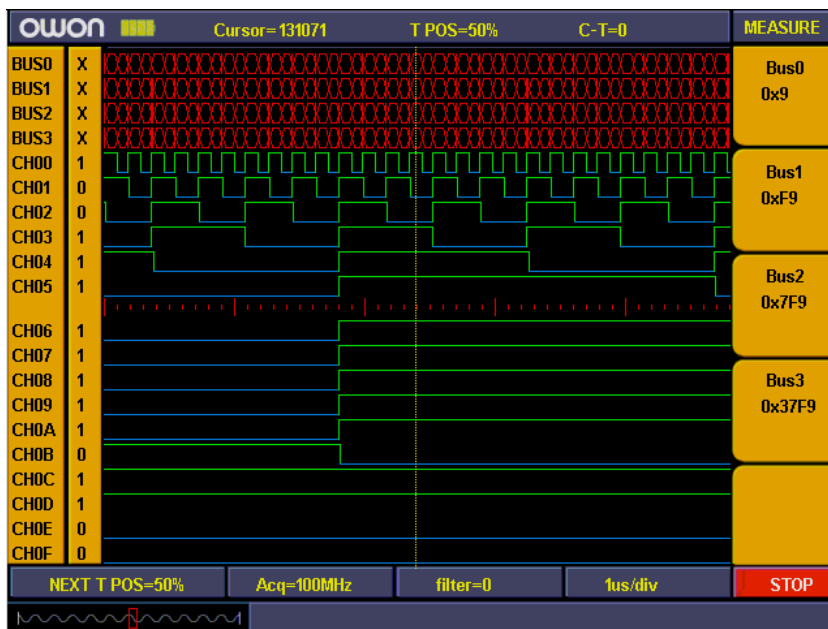
Fig 80: Bus measurement
