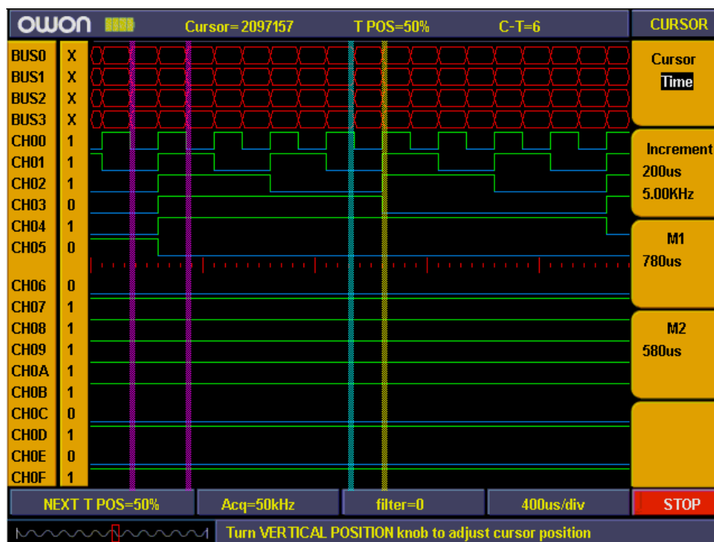
Fig 88: Cursor time measurement
