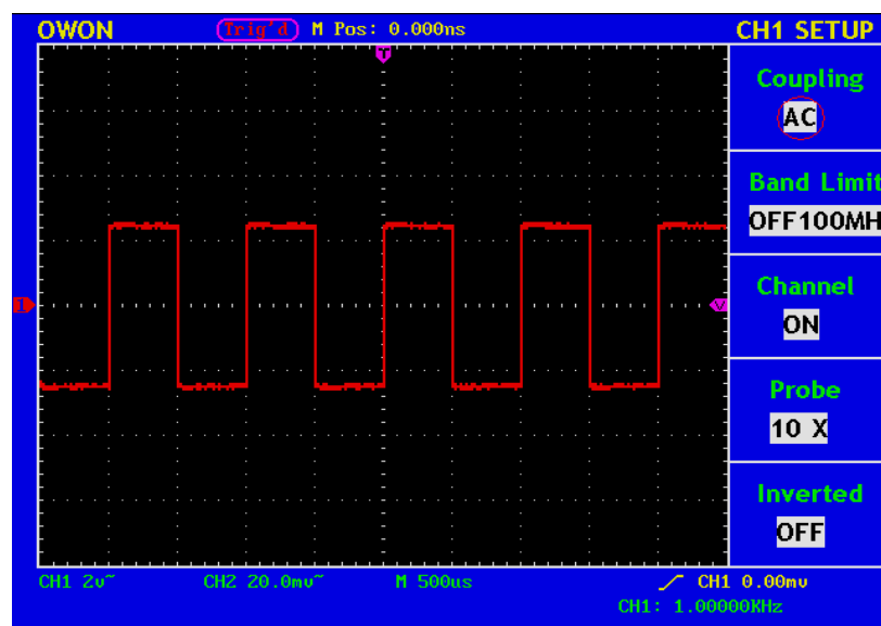
Fig. 21 AC Coupling Oscillogram
