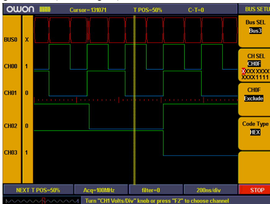
Fig 79: Bus setting
