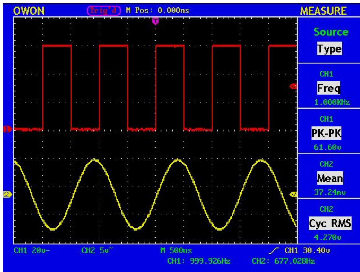
Fig. 56 Automatic Measurement
