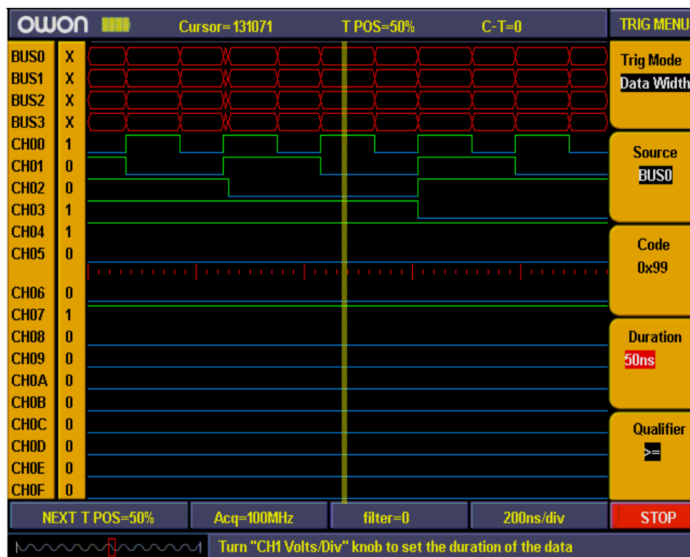
Fig 73: Data width trigger
