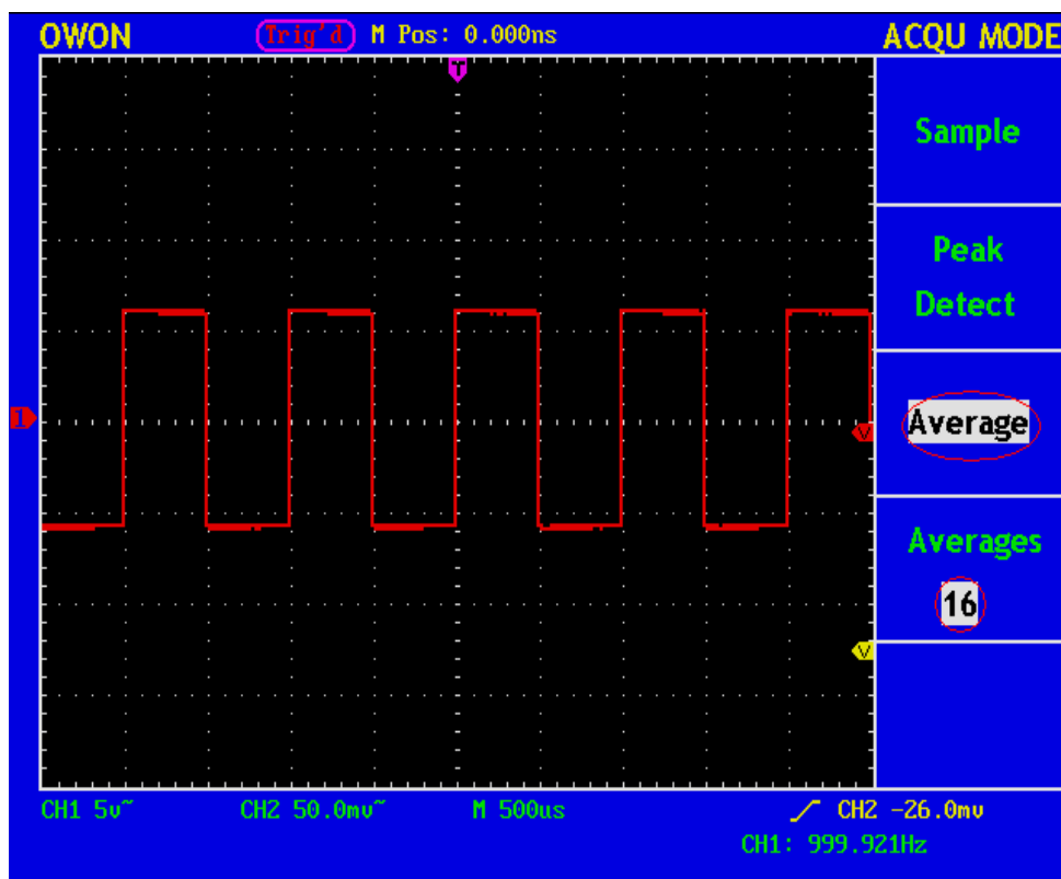
Fig. 44 The displayed wave form after the noise is removed under the Average Mode, in which the average number of 16 is set.
