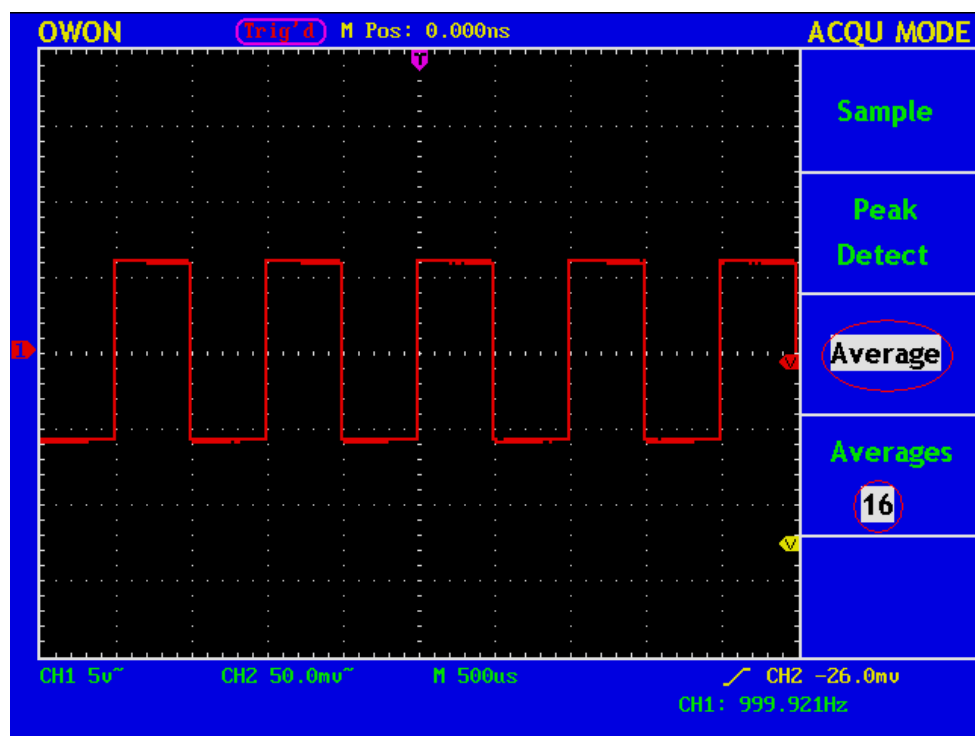
Fig. 94 Wave Form of the Noise-Removed Signal
