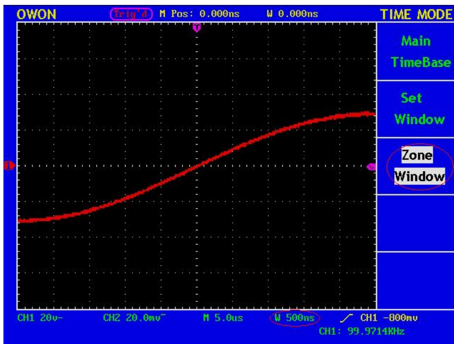
Fig. 31 Zone Window
