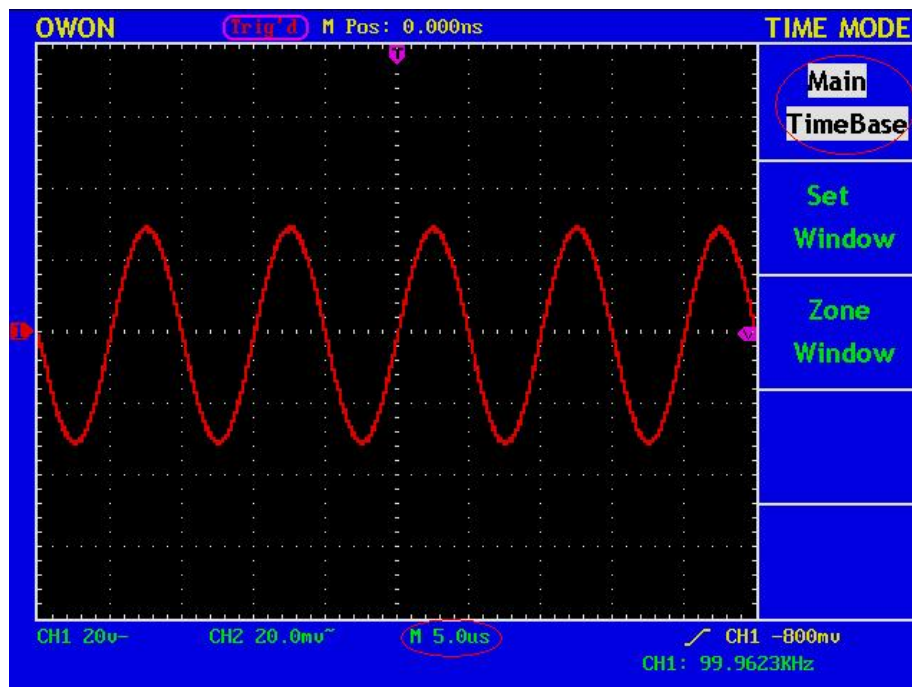
Fig. 29 Main Time Base
