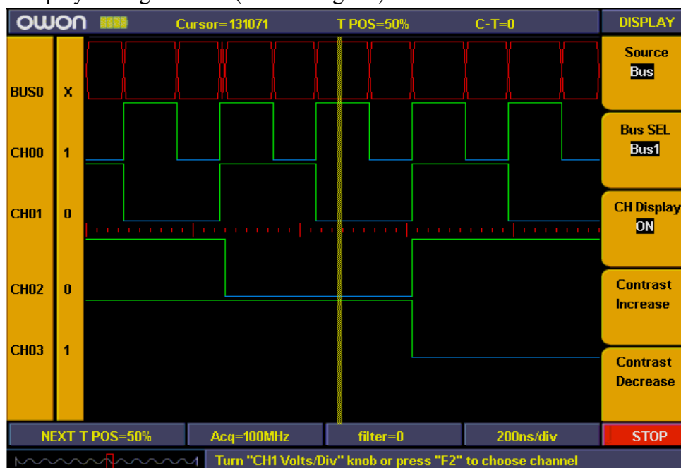
Fig 77: Display setting
