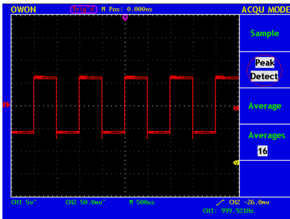
Fig. 93 Wave Form of the Signal Containing Noises
