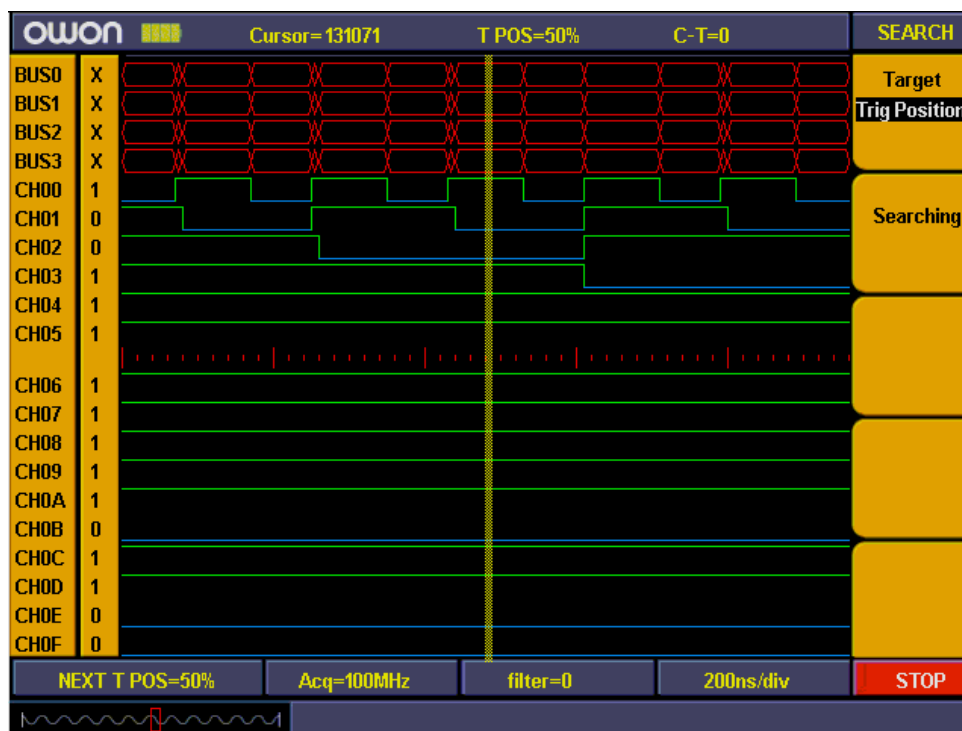
Fig 83: Search trigger position
