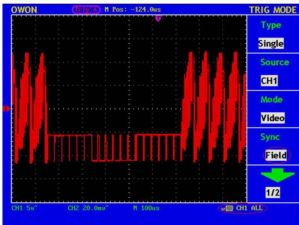
Fig. 96 Wave Form Obtained from Video Field Trigger
