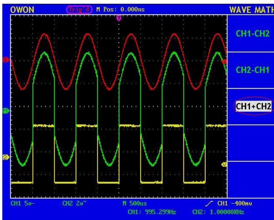
Fig. 26 Wave Form resulted from CH1 +CH2 Mathematical Manipulation
