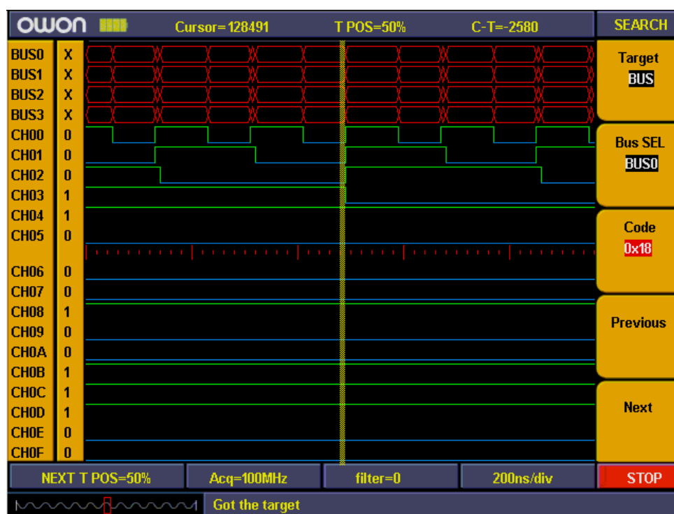
Fig 84: Search Bus
