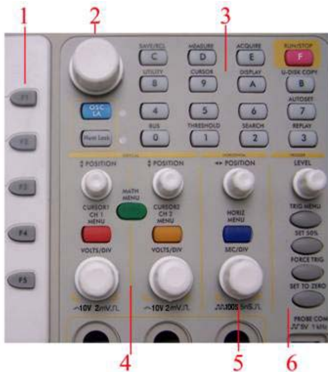
Fig 2: Keys Overview
