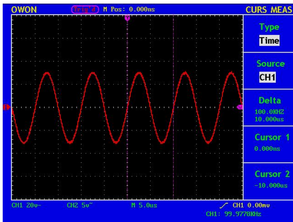
Fig. 59 Wave Form of Cursor Measurement
