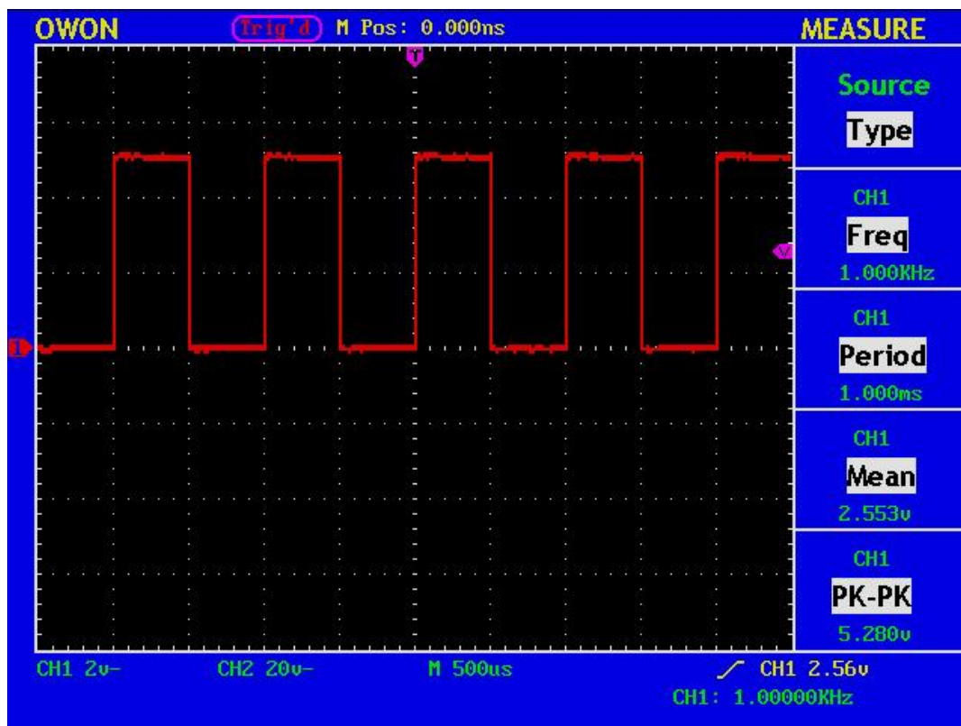
Fig. 90 Waveform of Automation Measurement
