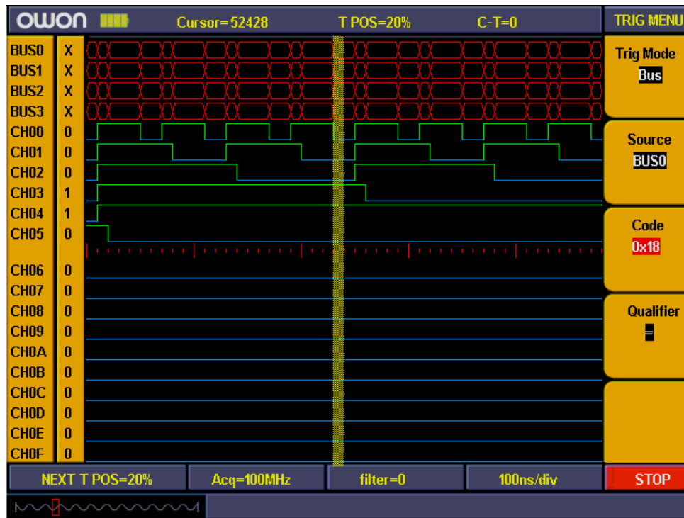
Fig 65: Bus trigger
