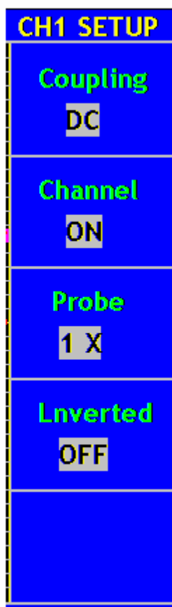
Fig. 14 Channel Setting Menu
