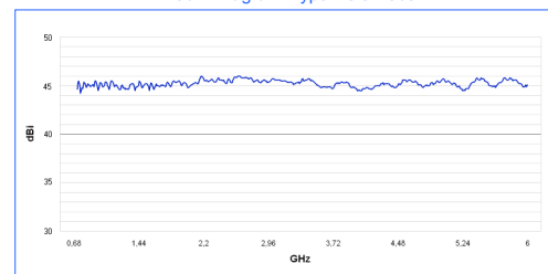
Gain Diagram HyperLOG 7060X
