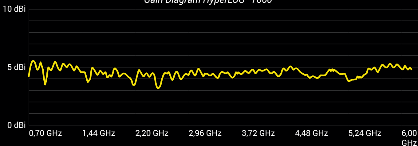
Gain Diagram HyperLOG® 7060
