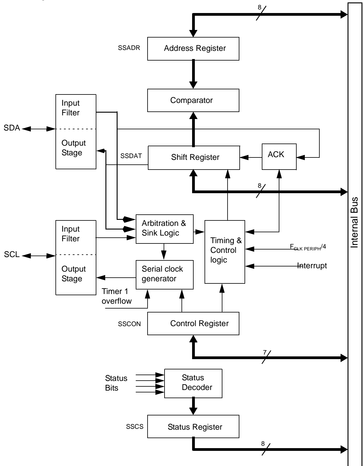
Figure 49. Block Diagram
