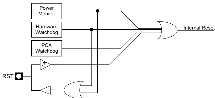
Figure 71. Reset schematic
