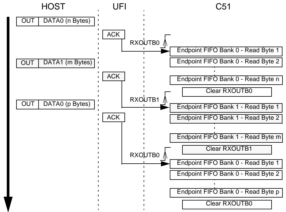
Figure 62. Bulk/Interrupt OUT Transactions in Ping-pong Mode
