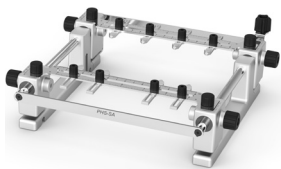
Small PCB Support ..... 1 unit Ref. PHS-SA
