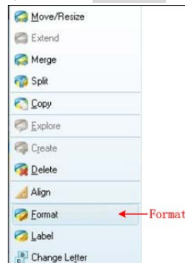
Figure 4-11: Choose format
