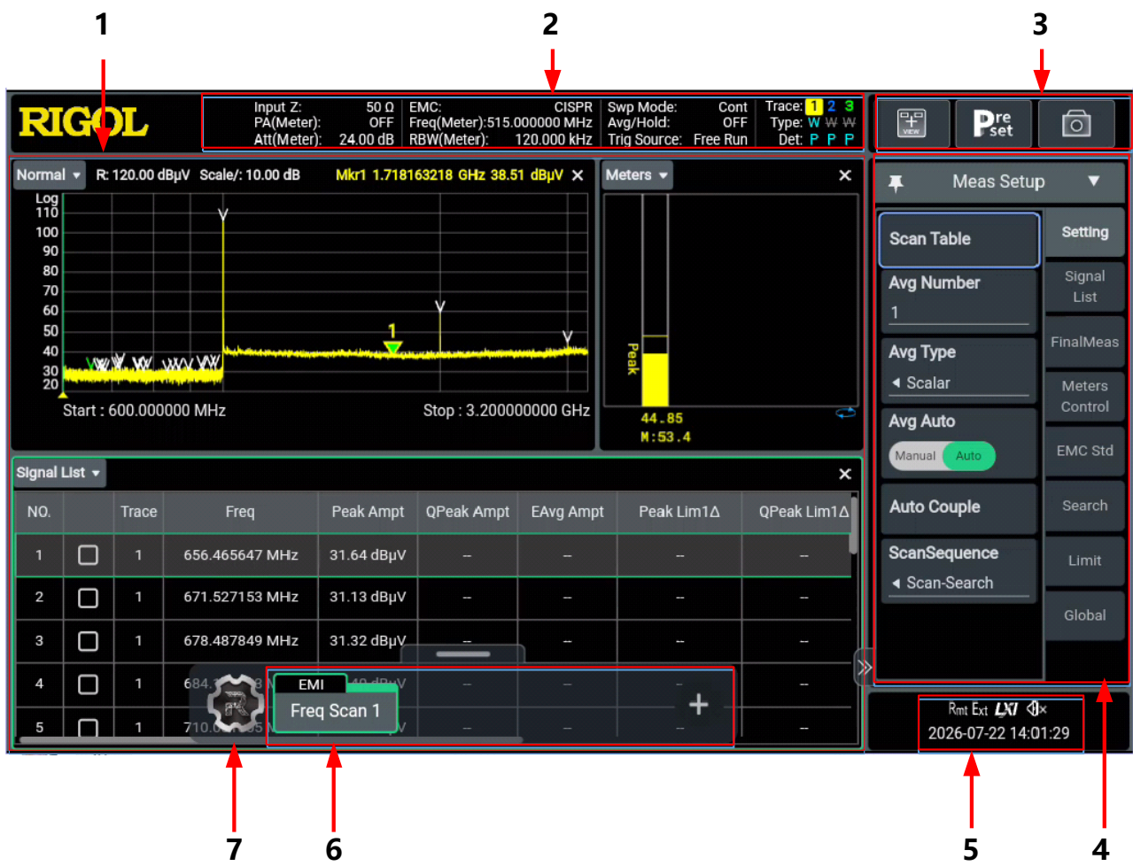
Figure 4.1 User Interface
