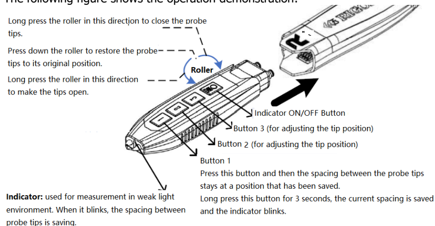
Figure 10 How to Operate the Hand-held Differential Probe Head
