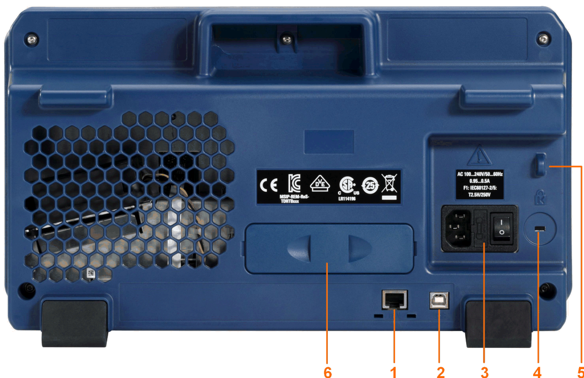
Figure 4-2: Rear panel view of R&S RTB 2
