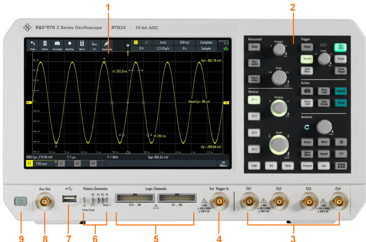
Figure 4-1: Front panel of R&S RTB24 with 4 input channels
