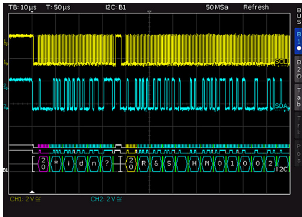
Figure 11-4: I2C bus
