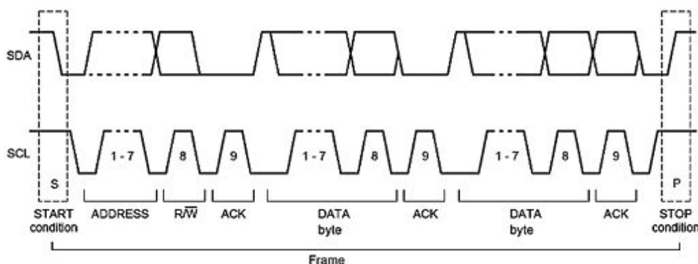
Figure 11-3: I 2 C 7-bit address
