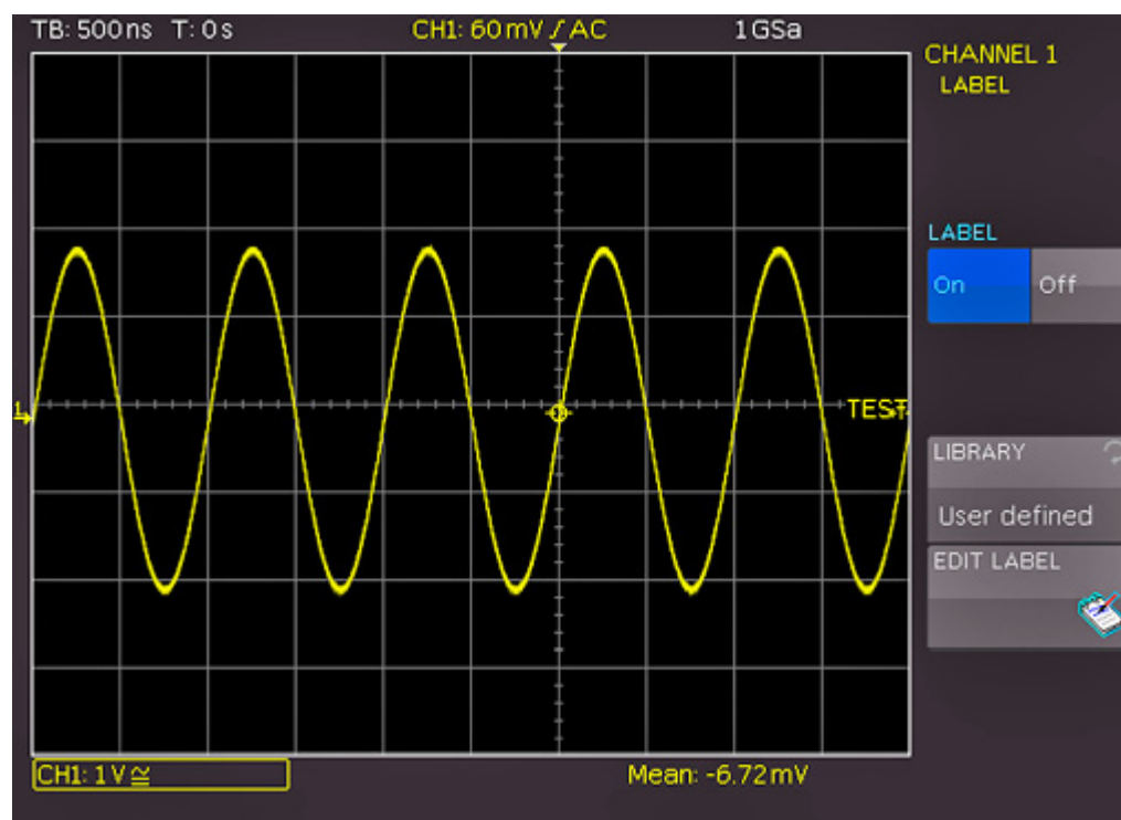
Figure 4-3: Label menu
