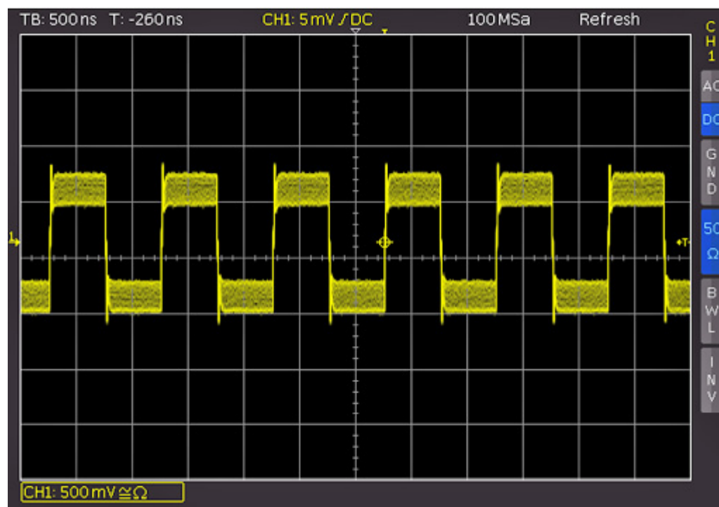
Figure 4-4: AM modulated signal with maximum repeat rate
