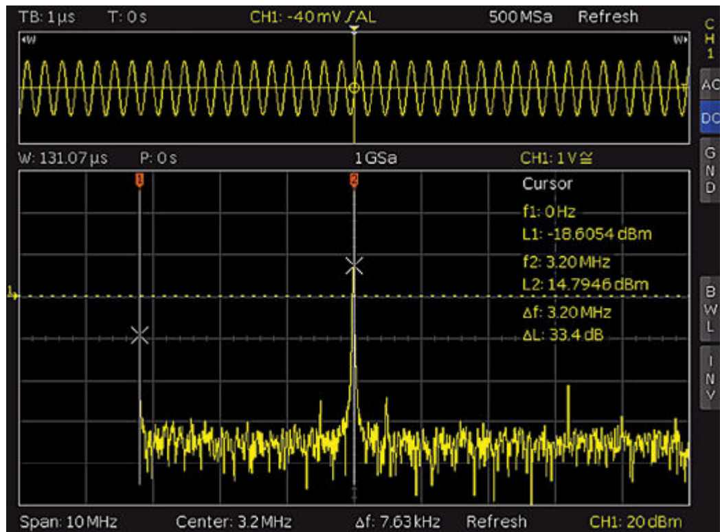
Figure 6-12: FFT
