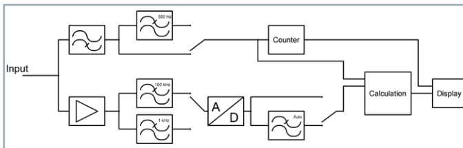
Abb. 6.29: Filterkette
