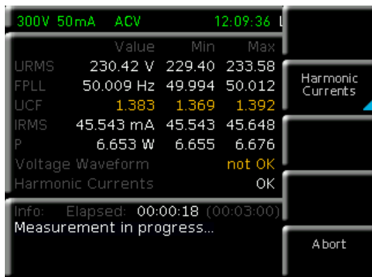
Abb. 6.19: Compliance Test Messung IEC 61000-3-2
