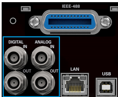
Abb. 6.31: BNC-Anschlüsse Digital / Analog IN/OUT
