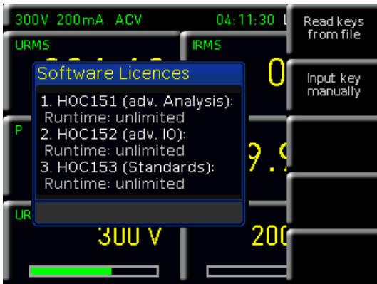
Abb. 3.1: Upgrade Menü
