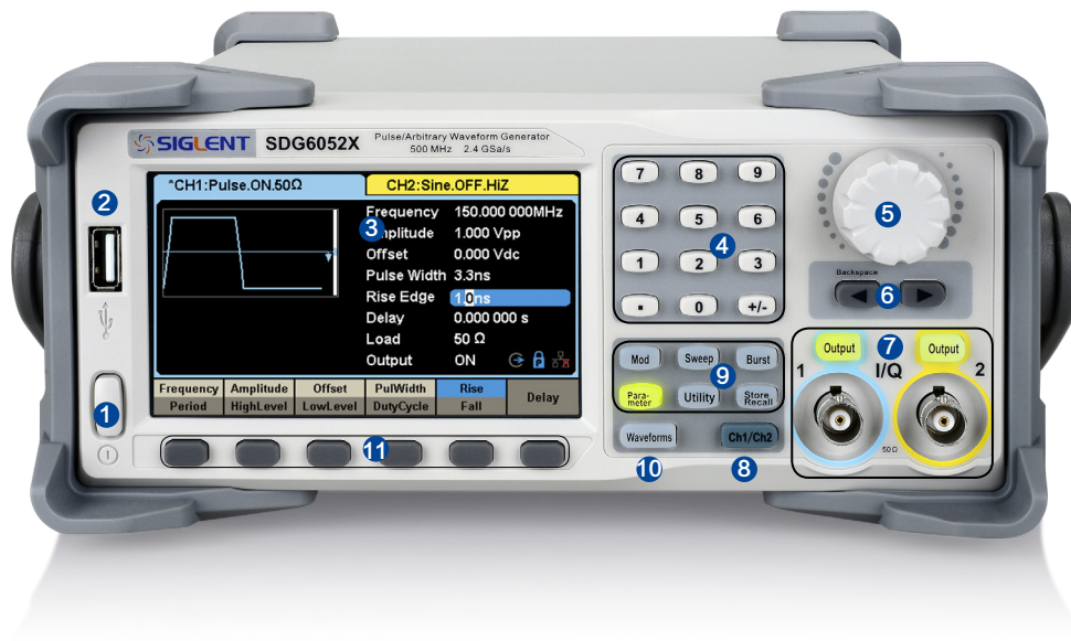
Figure 2 SDG6000X Front Panel
