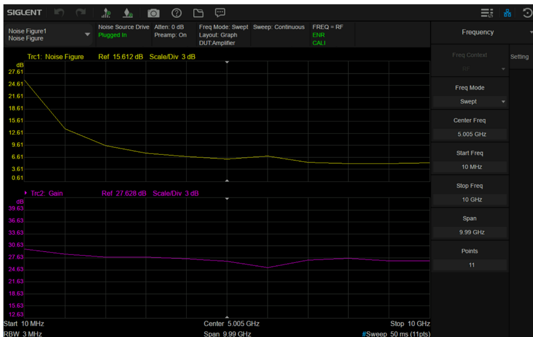
Figure 1-7 Noise figure measurement result
